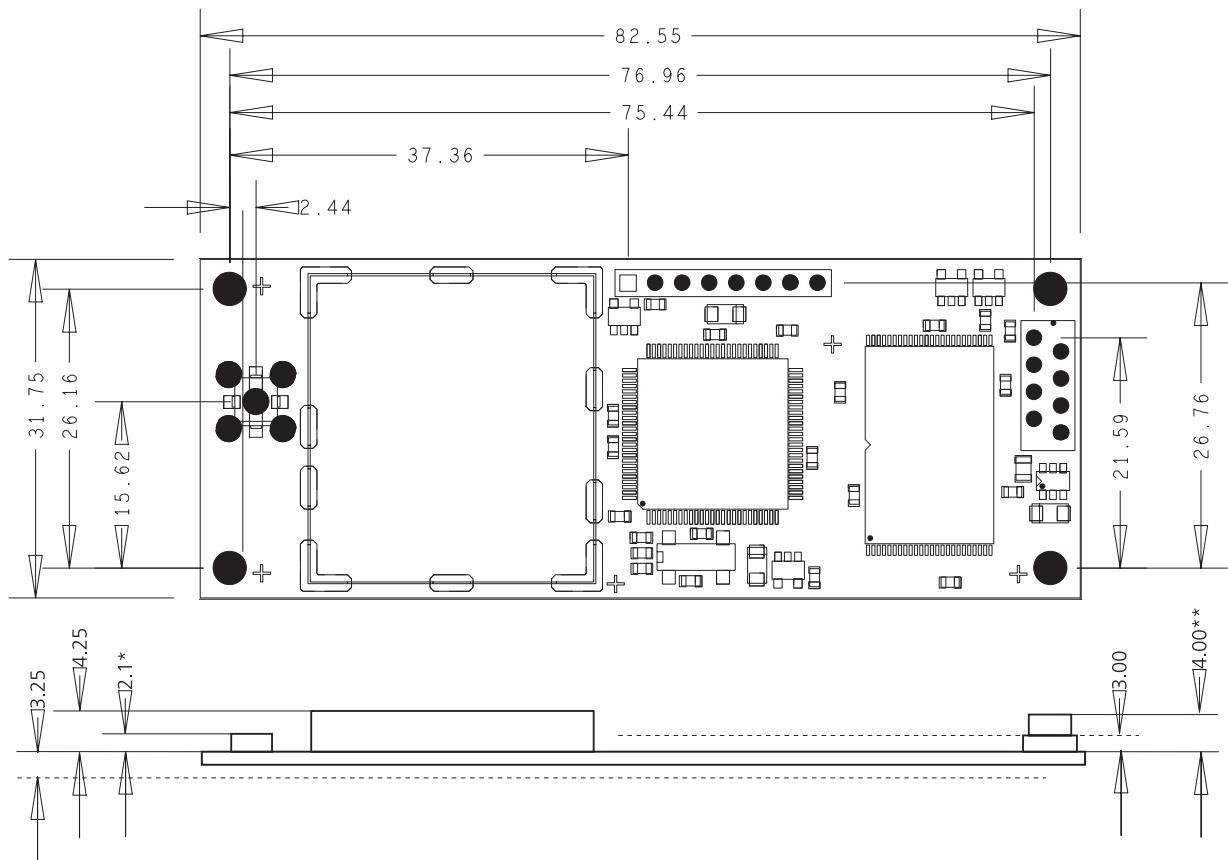
TOP View GPS-PS1 (with SSMT Connector)
