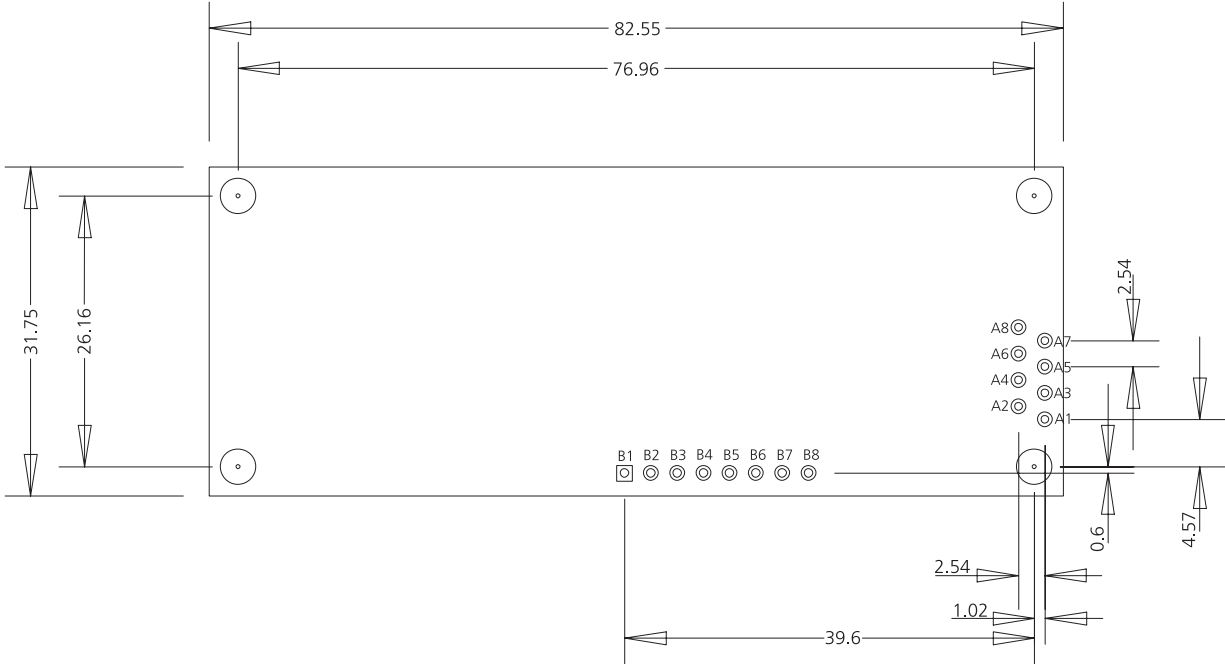
Figure 4: Recommended Footprint
