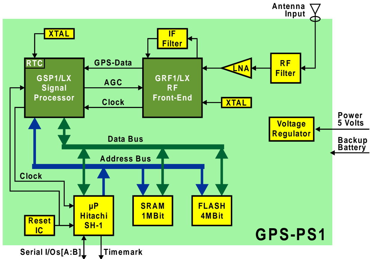
Figure 1: Blockdiagram of GPS-PS1
